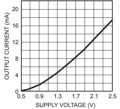
Short Circuit Current vs Supply Voltage Sourcing
